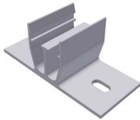
2 Flange Connection * Shown without butyl option (2) #14-13 X 3" Concealor™ screws
