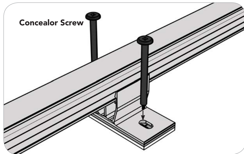
2 Flange Connection Option
